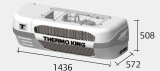
EV-580/ EV-580S Condenser
